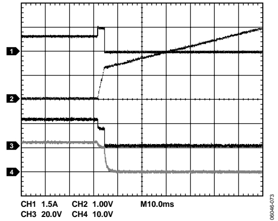
Figure 44. Overcurrent Condition During Operation (ADM1176-1 Model) (Channel 1 = I_{LOAD} , Channel 2 = V_{TIMER} , Channel 3 = V_{GATE} , Channel 4 = V_{OUT} )
