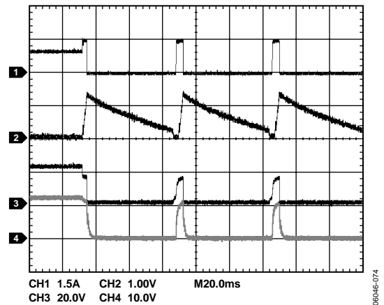
Figure 45. Overcurrent Condition During Operation (ADM1176-2 Model) (Channel 1 = I_{LOAD} , Channel 2 = V_{TIMER} , Channel 3 = V_{GATE} , Channel 4 = V_{OUT} )
